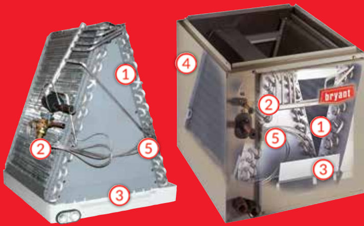
Model CAPVU Vertical Uncased A-Coil
